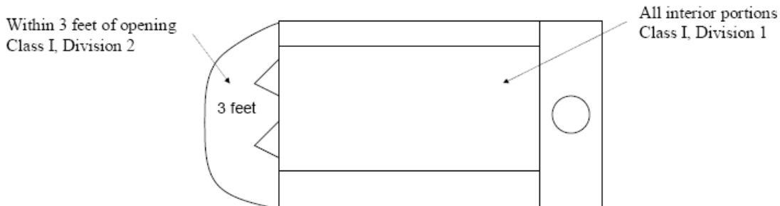
Typical Enclosed Vehicle Spray Booth (plan view)
